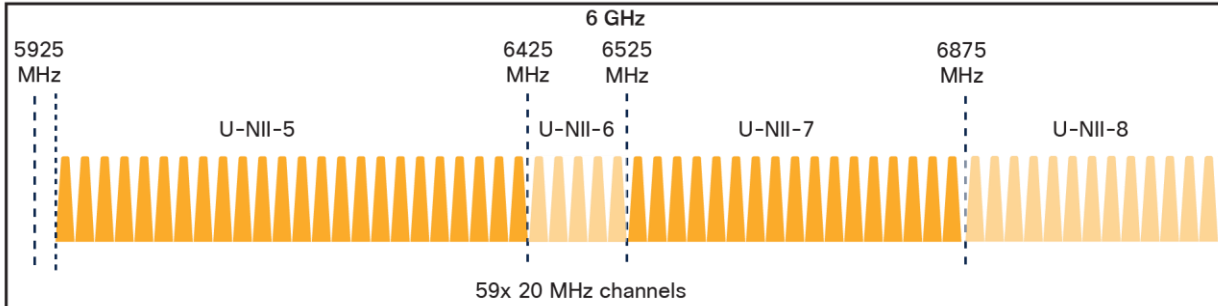
Figure 28. Depiction of 6-GHz spectrum
