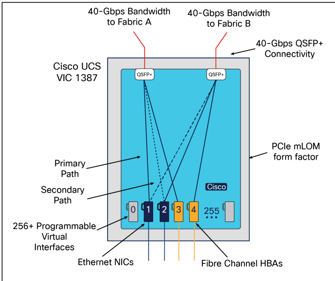
Figure 3. Cisco UCS VIC 1387 Architecture
