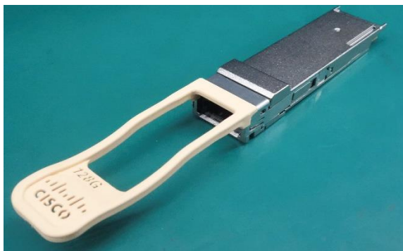
Figure 14. Cisco 128-Gbps Fibre Channel QSFP Transceivers
