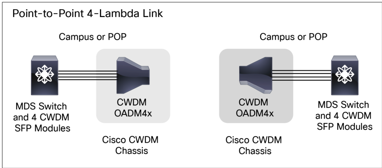
Figure 17. Point-to-Point Architecture (Dual-Fiber Link)
